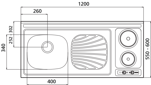
Dimensions (mm): Dimensiones (mm):
